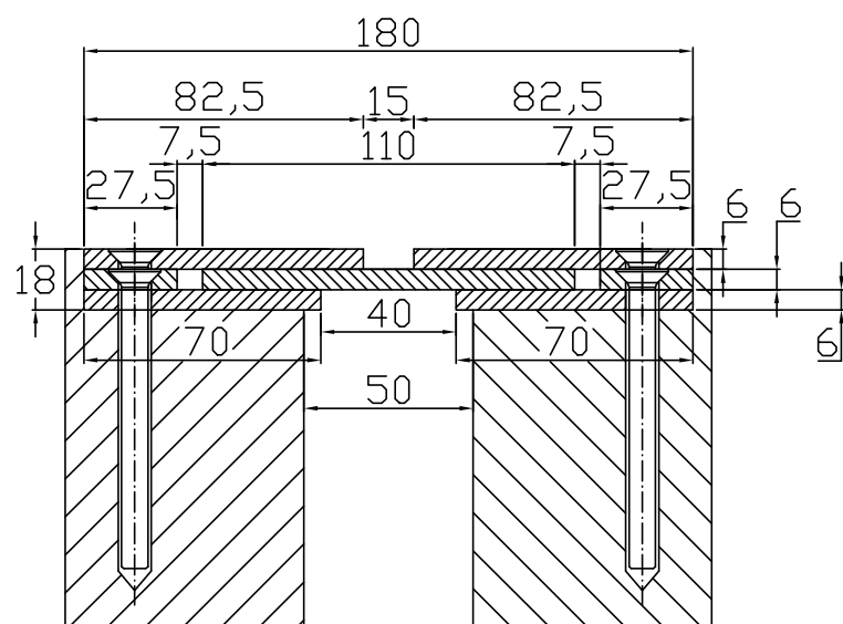
Conecto Sinus 06NC180/18-R S50K15 Section
