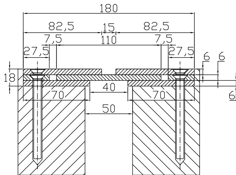
Conecto Sinus 06NC180/18-R S50K15 Section
