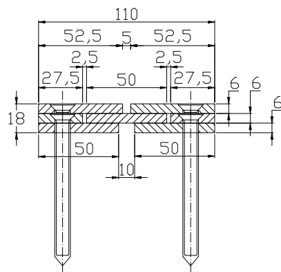
CONNECTO SINUS 06NC110/18-R S10K5 Section
