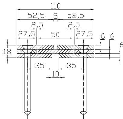
Conecto Sinus 06NC110/18-R S10K5 Section
