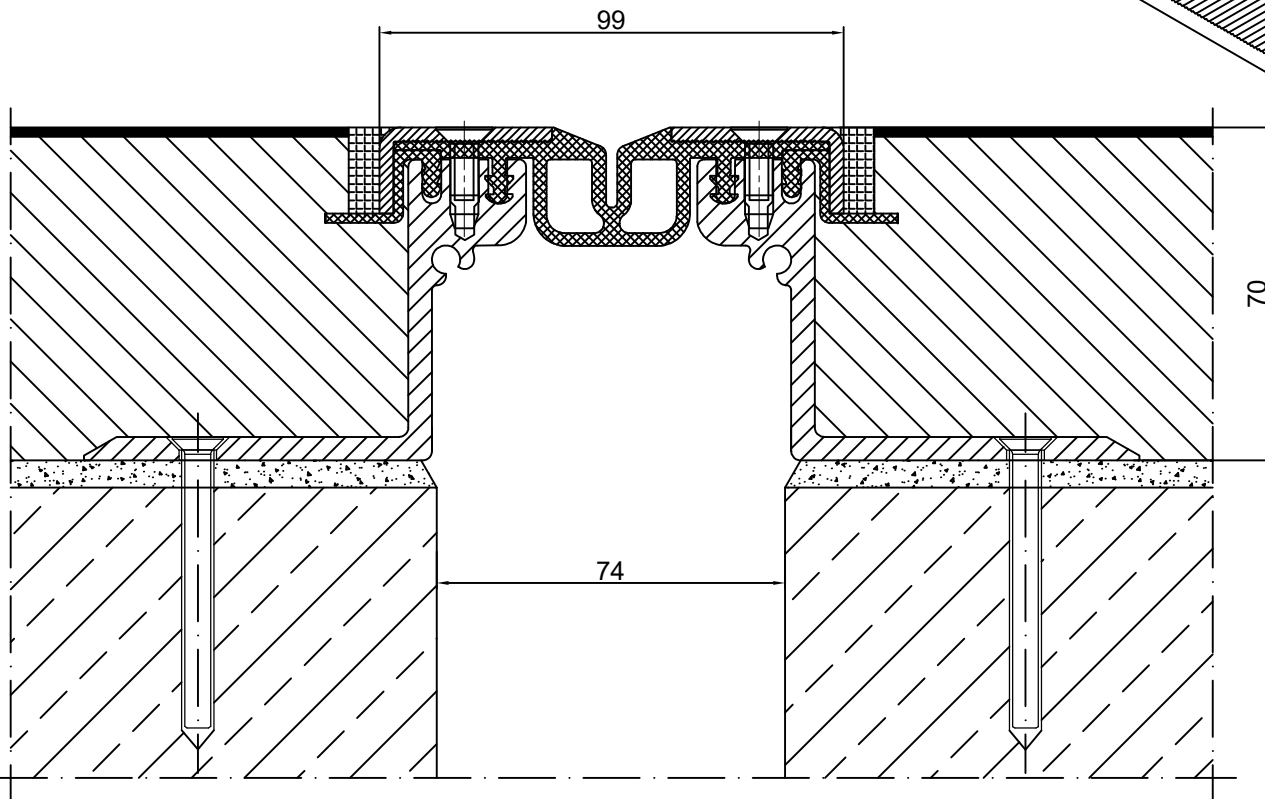
CONECTO GA 50.20.70 S SECTION
